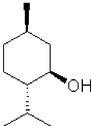
(-)-1R,3R,4S-MENTHOL
